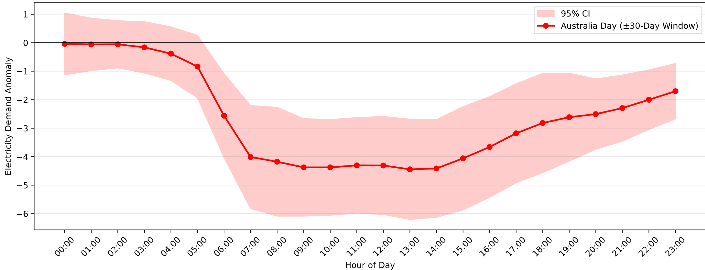
Leightonfield Demand Anomaly: Australia Day (2004–2017, \pm 30 -Day Window)
